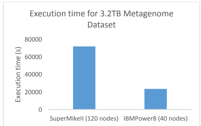
Figure 6: Execution time for 3.2TB
