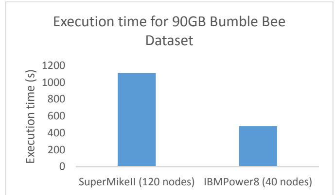
Figure 5: Execution time for 90GB Bumble Bee genome
