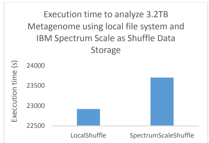
Figure 8: Performance comparison between local file system and Spectrum Scale as shuffle data storage
