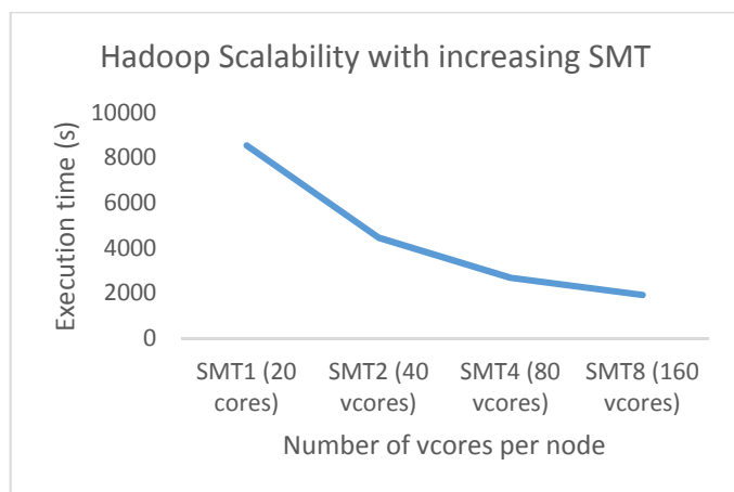
Figure 3: Scalability of Hadoop with increasing SMT
