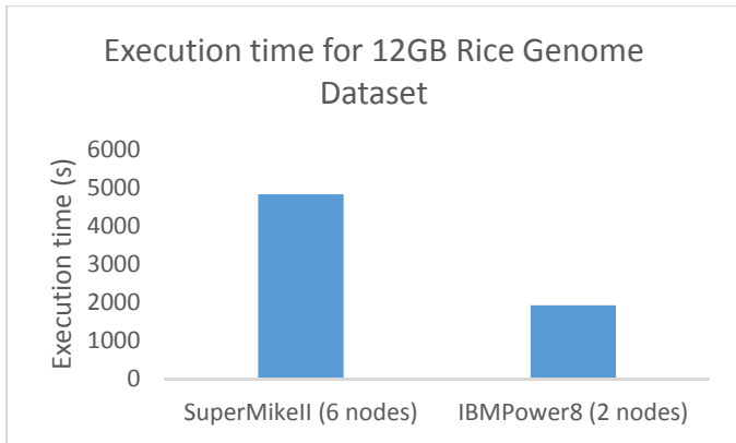
Figure 4: Execution time of Rice genome
